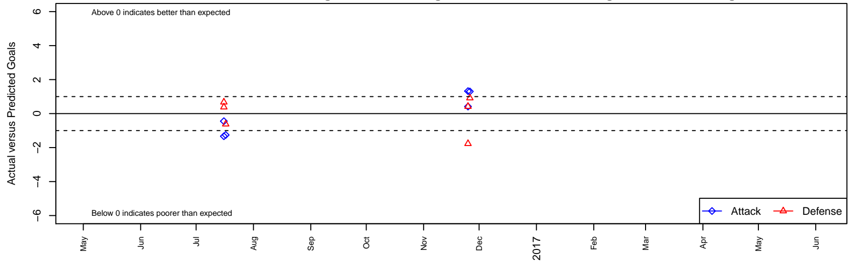
San Diego United Black B99 Dots are actual minus expected GF (blue circles) and GA (red triangles). Blue line is smoothed change in attack strength. Red is smoothed change in defense strength.
